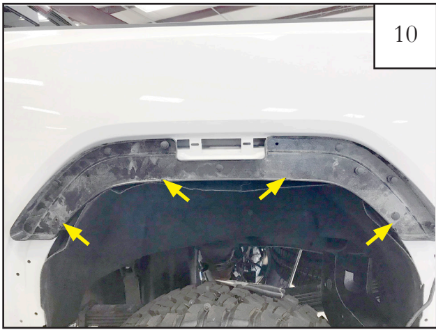
Use (4) U-clips (CL1-0022) installed at (4) hole locations on inner bracket.
