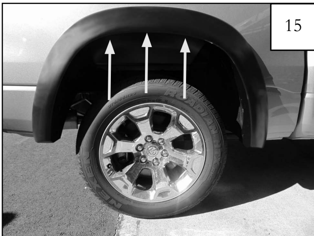
Hold flare in place and start Screw (SW1-0056) using a Phillips screwdriver in (3) locations as shown. Do not tighten. Continue to Step 18.
