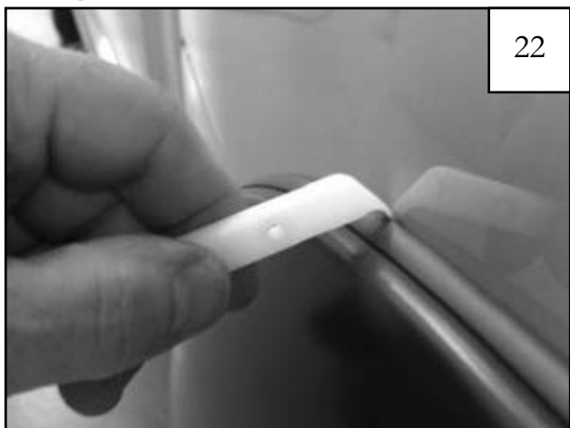
22 Using supplied Edge Trim Tool (ET1-0002), seat edge trim against vehicle by hooking curved end under edge trim at one end of flare. Next, slide around outer edge of flare to the other end.
