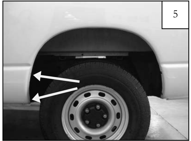
Install Clip (CL1-0011) in these locations. See step 6.
