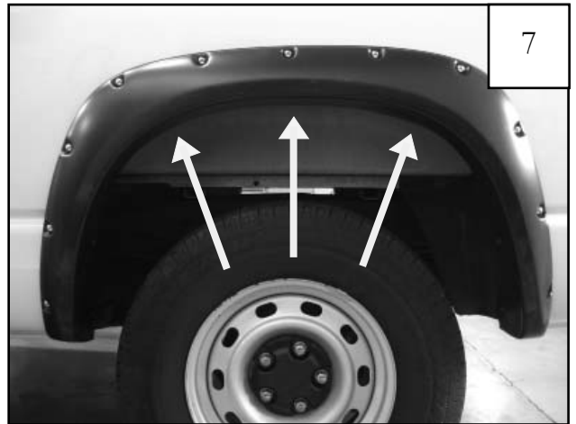
Hold flare in place and mark three locations with a grease pencil using the holes in the flare as a guide. See steps 8 & 9.
