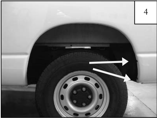
Remove two factory installed screws using an 8mm socket wrench. Keep screws for installation of the rear flare.
