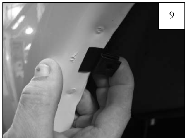
Slide a Clip (CL1-0005) over each Tab (MT1-0014).
