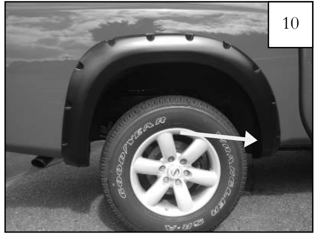
Passenger Side Flare: Hold (RR) flare in position on fender with moderate pressure. Line up the lowest hole in fender with the hole in flare and start the factory screw. Do not fully tighten screws.
